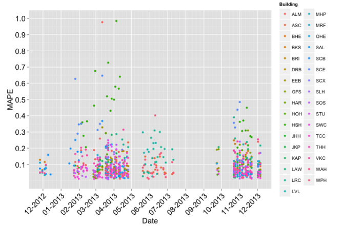
Figure 9: MAPE error per event event per building.
